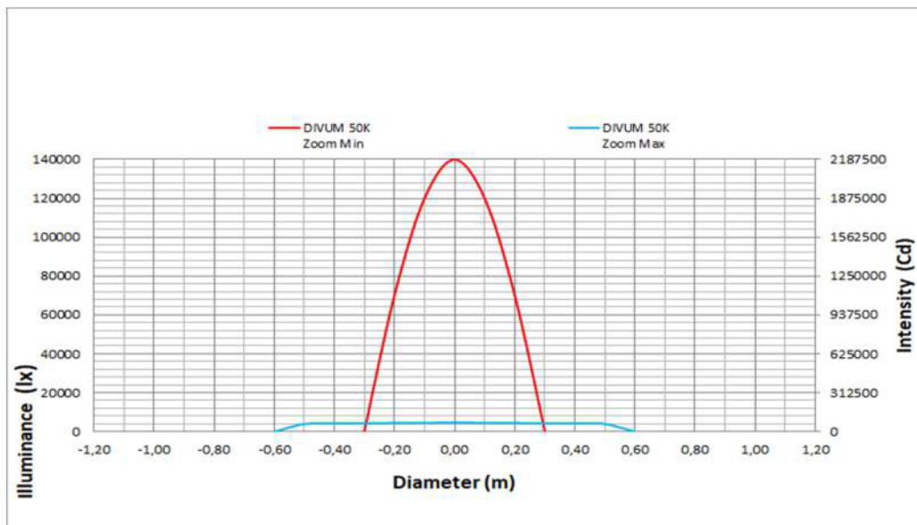
Illuminance distribution DIVUM 50K
