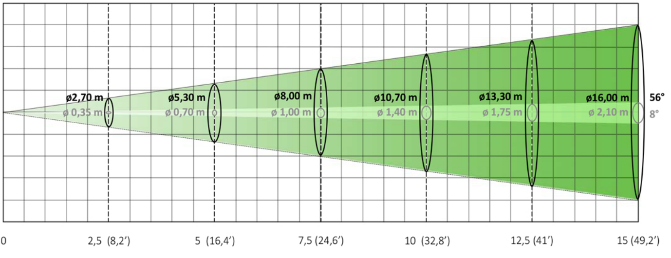
Illuminance distribution DIVUM 50K
